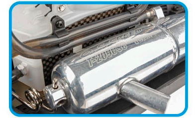
RC8B4.1 fuel tank with flexible rubber lid puller, tight seal spring and official ONG fuel tank guard
