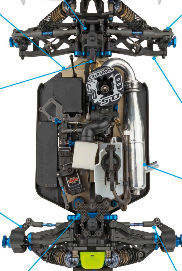
New durable rear hub design with wide footprint base, and tuneable 3mm carbon fiber tall hub towers
